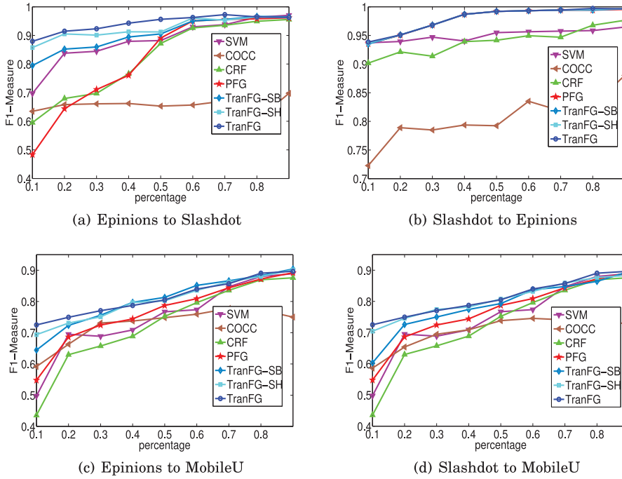
Fig. 14. Performance of predicting friendships with and without the balance- and structural-hole-based transfer by varying the percentage of labeled data in the target network.
