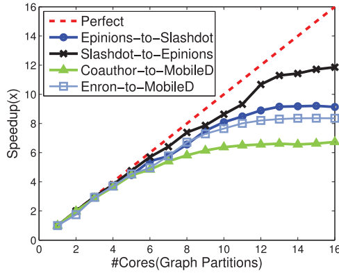
Fig. 3. Speedup versus #cores.
