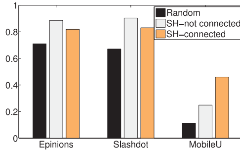
Fig. 6. Structural hole. SH-connected and SH-not connected respectively represent the probability that two connected and two disconnected users (A and B) have the same type of relationship with user C, conditioned on user C spanning a structural hole. “Random” indicates the average probability that two users (A and B) have the same type of relationship with user C regardless of whether C spans a structural hole. It is clear that users are more likely (on average +70% higher than chance) to have the same type of relationship with C if C spans a structural hole.
