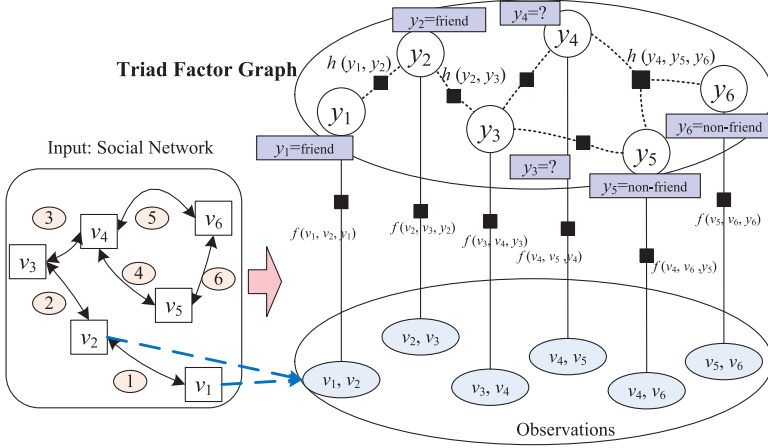
Fig. 11. Graphical representation of the triad factor graph (TriFG) model. Each ellipse indicates a relationship; for example, (v_1, v_2) represents a relationship between v_1 and v_2 . Notation \mathbf{x}_i indicates the attribute vector associated with the relationship (v_1, v_2) . For each relationship, we use a corresponding latent variable y denoted as a circle to represent its type. Each black square denotes a factor function that takes the associated variables as input and outputs a real number.
