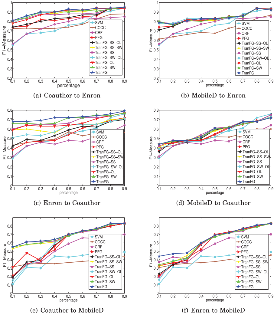
Fig. 15. Performance of predicting directed relationship with and without the status-, opinion-leader-, and strong/weak-tie-based transfer by varying the percentage of labeled data in the target network.
