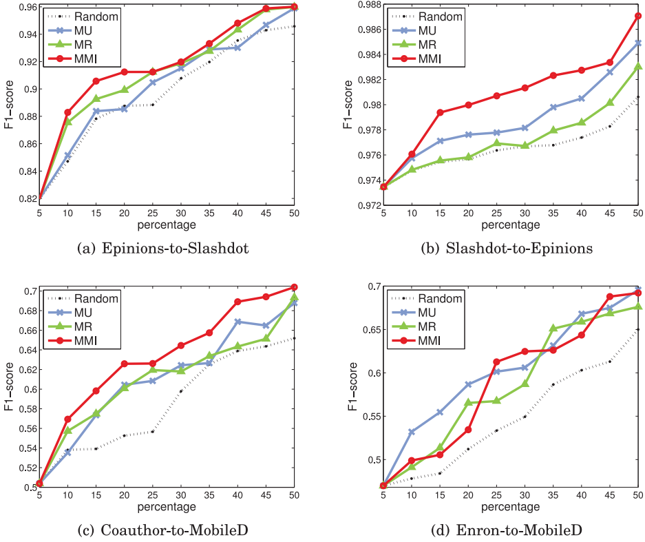
Fig. 2. Performance of active learning. MMI is our proposed method; Random, MU, and MR are three comparison methods.
