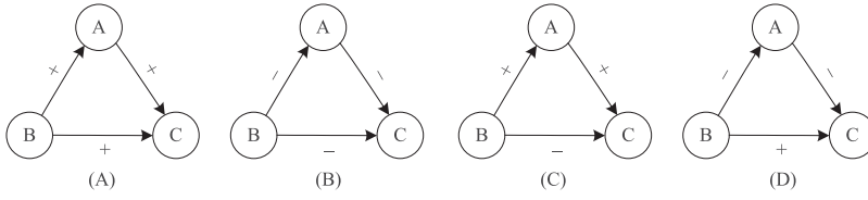
Fig. 7. Illustration of status theory. (A) and (B) satisfy the status theory, while (C) and (D) do not satisfy the status theory. Here, positive “+” denotes that the target node has a higher status than the source node, and negative “-” denotes that the target node has a lower status than the source node. In total there are 16 different cases.
