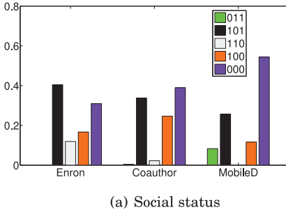
Fig. 8. Distribution of the five most frequent formations of triads with social status. Given a triad (A, B, C) , let us use 1 to denote the advisor-advisee relationship and 0 to denote the colleague relationship. The number 011 denotes that A and B are colleagues, B is C 's advisor, and A is C 's advisor.
