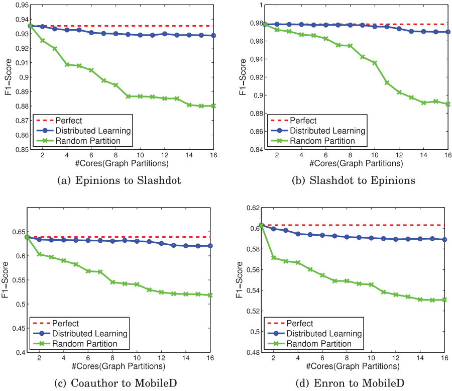
Fig. 17. Prediction accuracy (F1-score) by the distributed learning. The red dashed line is the accuracy performance on a single machine.
